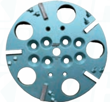
Dia. Floor Polish Plate 250mm x 10PCD + 5 SEG.
