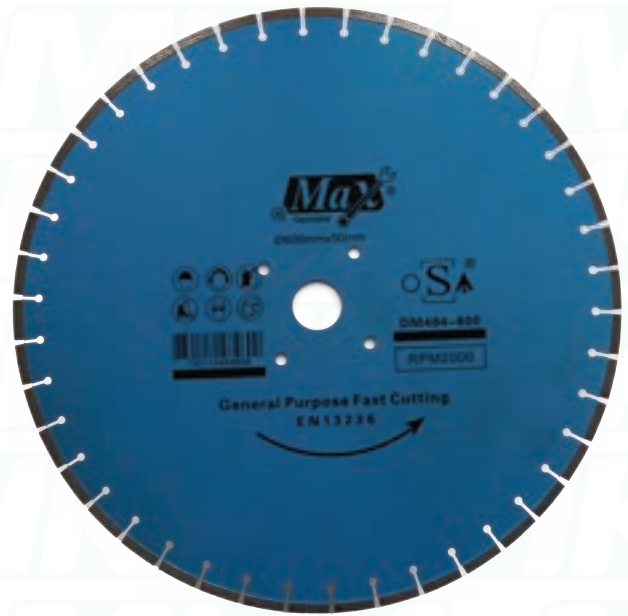
Concrete Normal 484 [50mm Hole]
