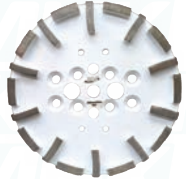
Dia. Floor Polish Plate 250mm x 20T #60
